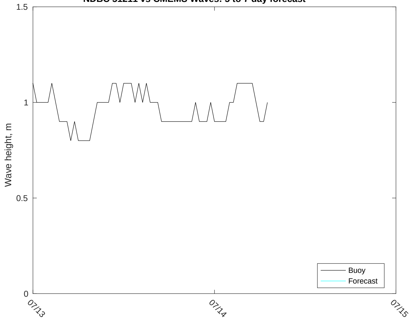
NDBC 51211 vs CMEMS Waves: 5 to 7 day forecast
