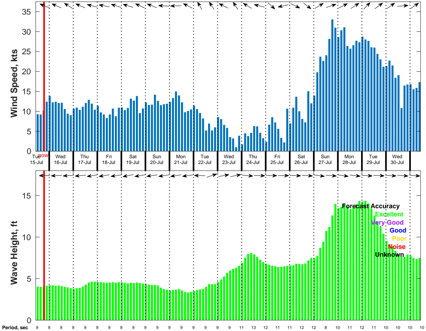
Wind & Wave Forecast for NDBC 52211 from 14-Jul-2025 11:00:00 to 30-Jul-2025 11:00:00
