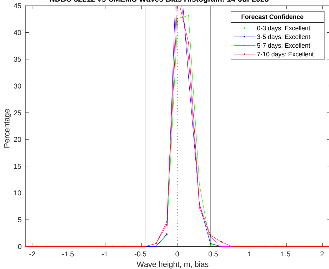
NDBC 52212 vs CMEMS Waves Bias Histogram: 14-Jul-2025
