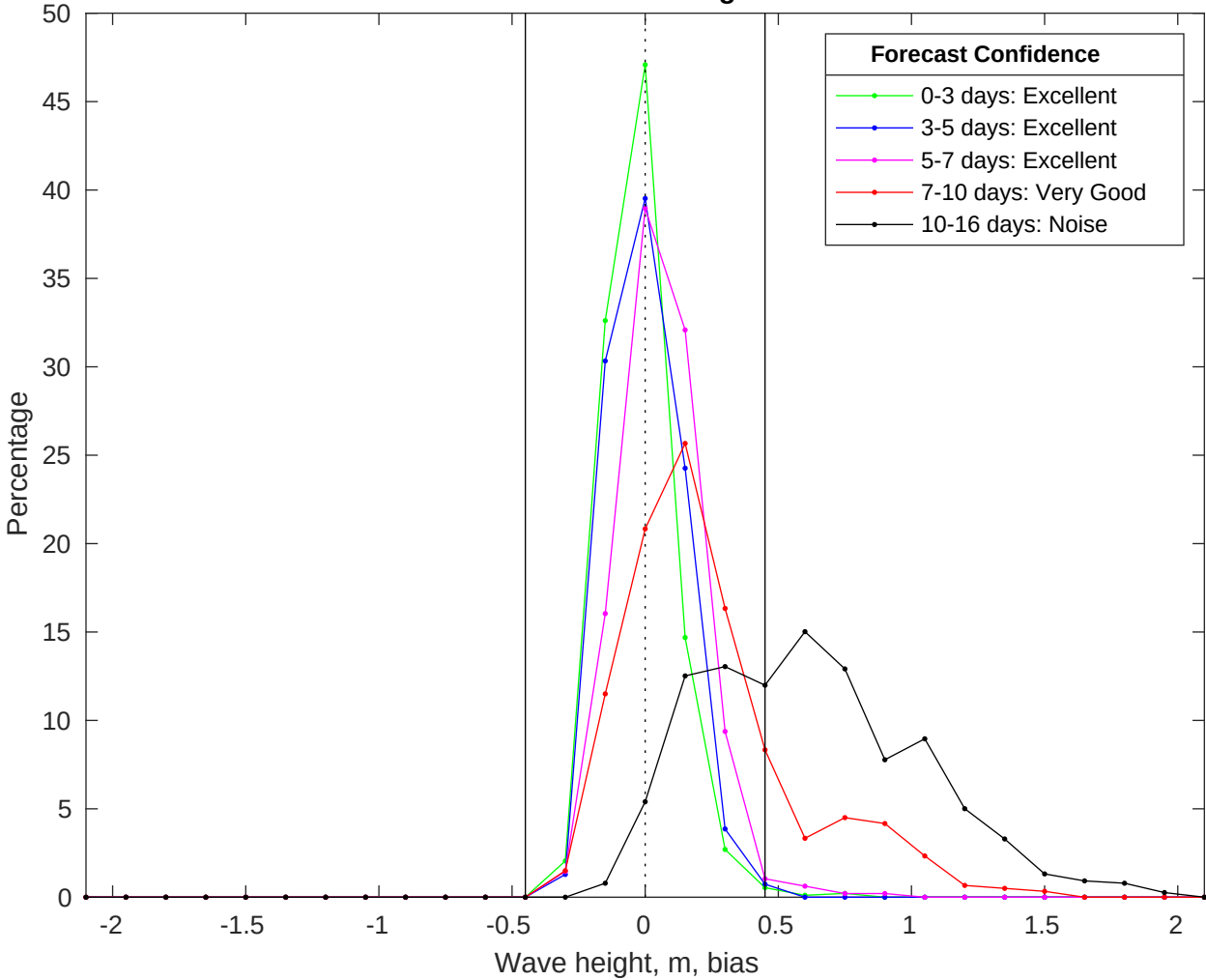
NDBC 52212 vs GFS Waves Bias Histogram: 14-Jul-2025
