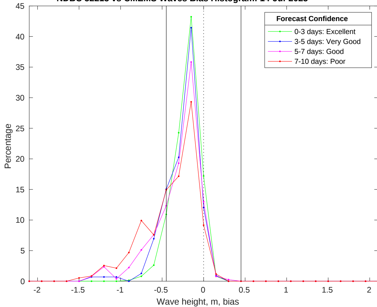
NDBC 52213 vs CMEMS Waves Bias Histogram: 14-Jul-2025
