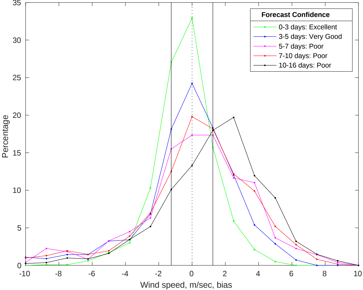
NDBC 41004 vs GFS Winds Bias Histogram: 15-Jul-2025
