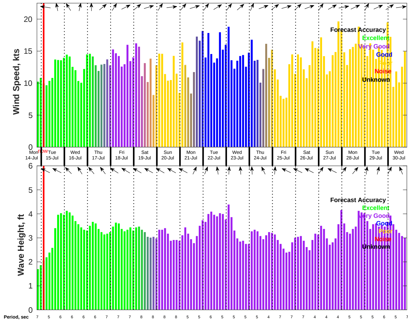
Wind & Wave Forecast for NDBC 41004 from 14-Jul-2025 19:00:00 to 30-Jul-2025 19:00:00
