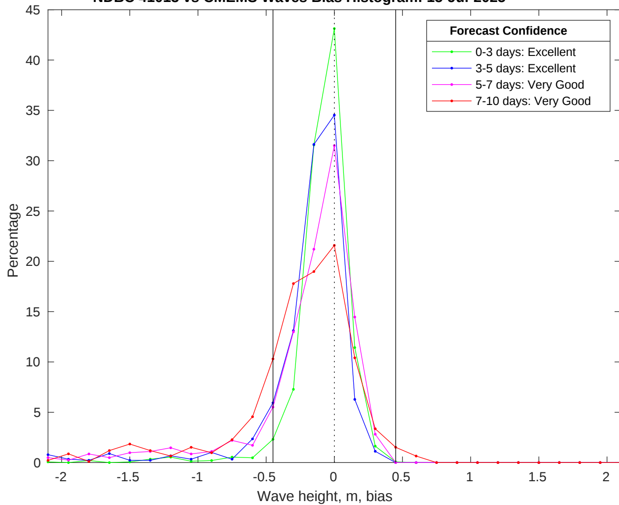
NDBC 41013 vs CMEMS Waves Bias Histogram: 15-Jul-2025
