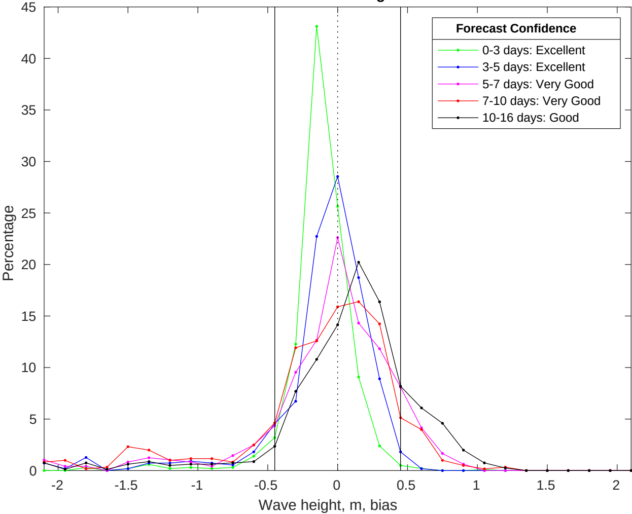
NDBC 41013 vs GFS Waves Bias Histogram: 15-Jul-2025
