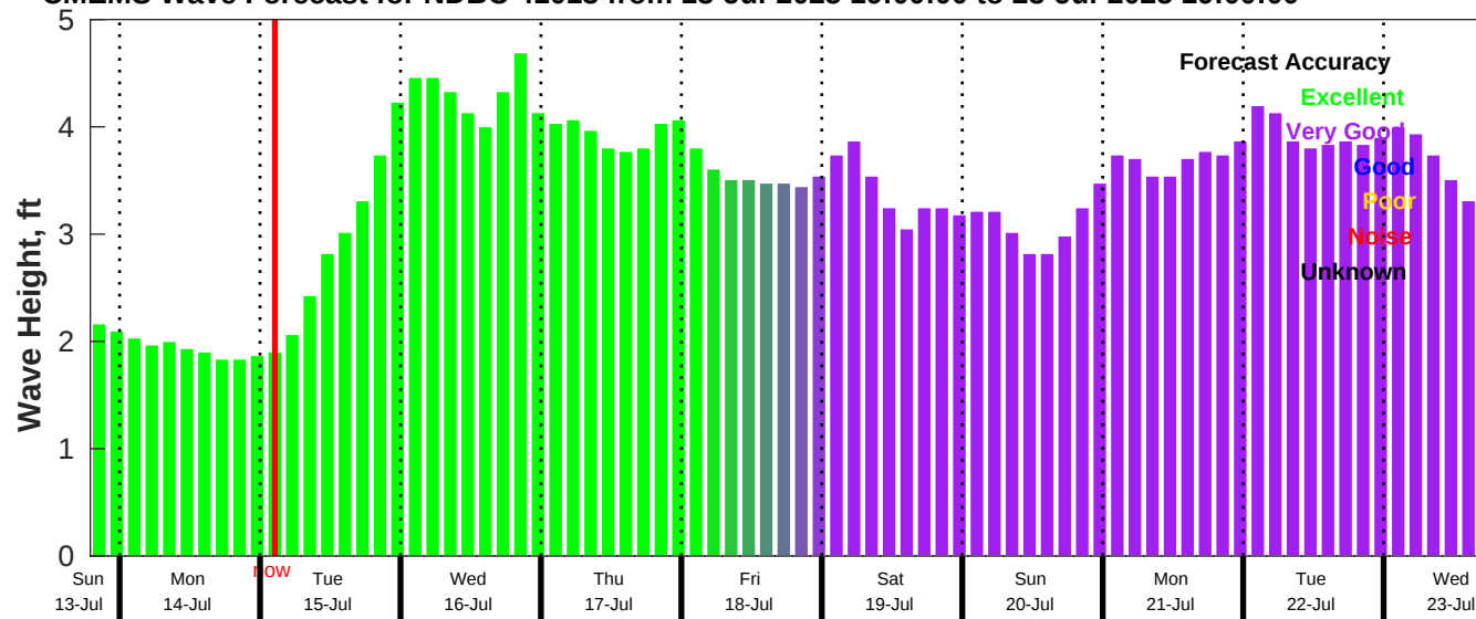
CMEMS Wave Forecast for NDBC 41013 from 13-Jul-2025 19:00:00 to 23-Jul-2025 19:00:00
