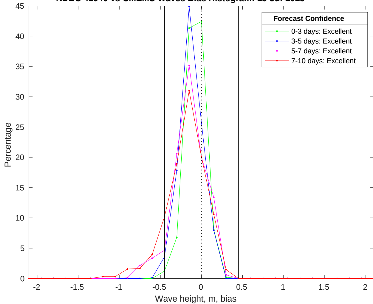
NDBC 41040 vs CMEMS Waves Bias Histogram: 15-Jul-2025
