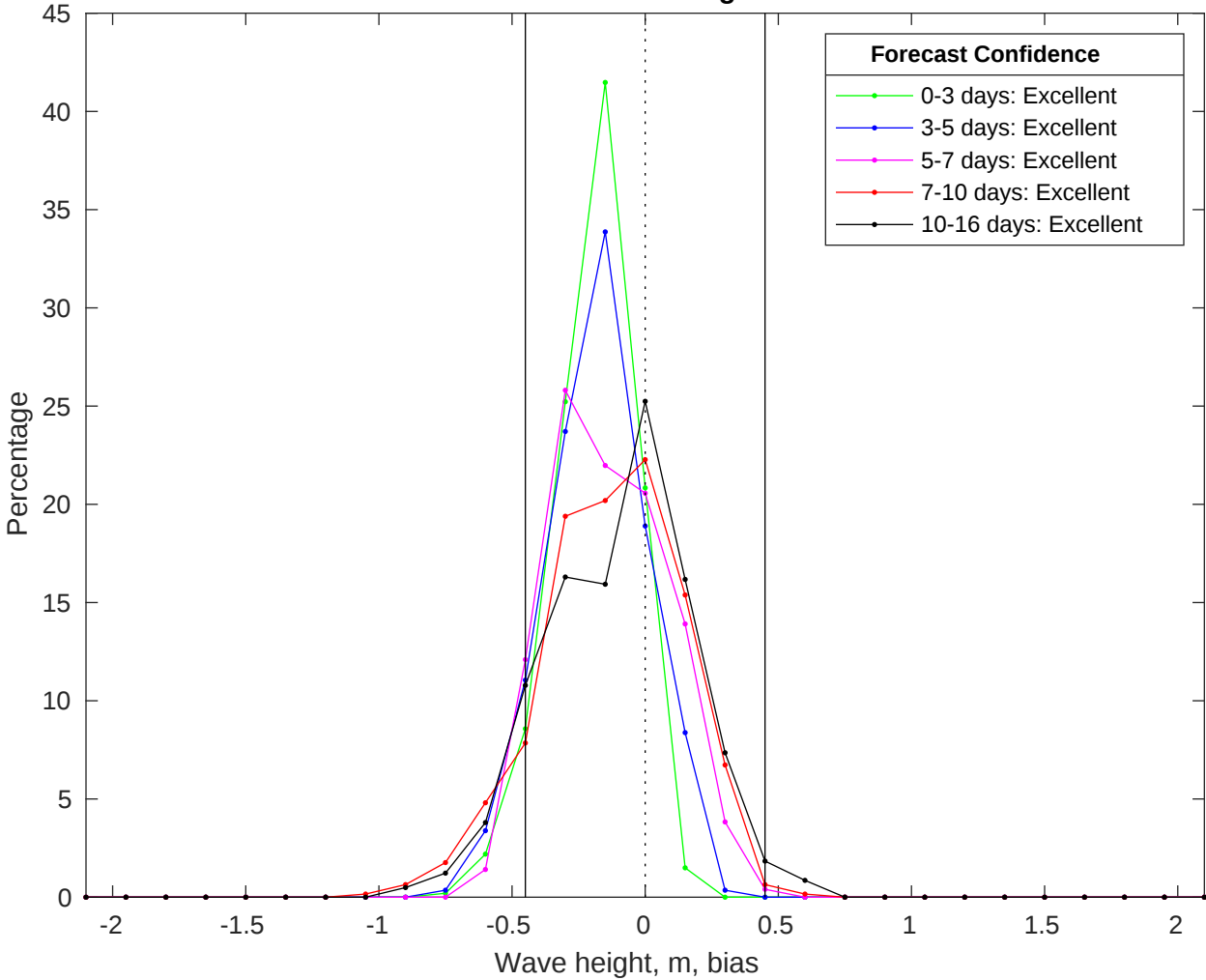
NDBC 41040 vs GFS Waves Bias Histogram: 15-Jul-2025
