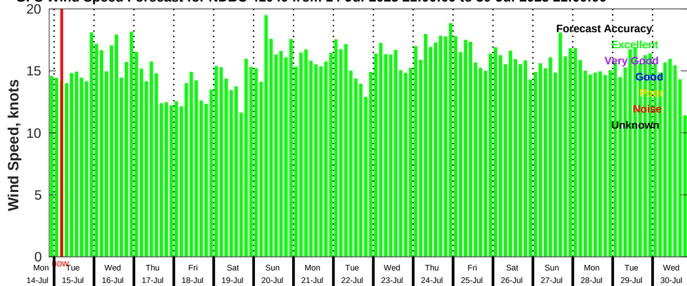
GFS Wind Speed Forecast for NDBC 41040 from 14-Jul-2025 21:00:00 to 30-Jul-2025 21:00:00
