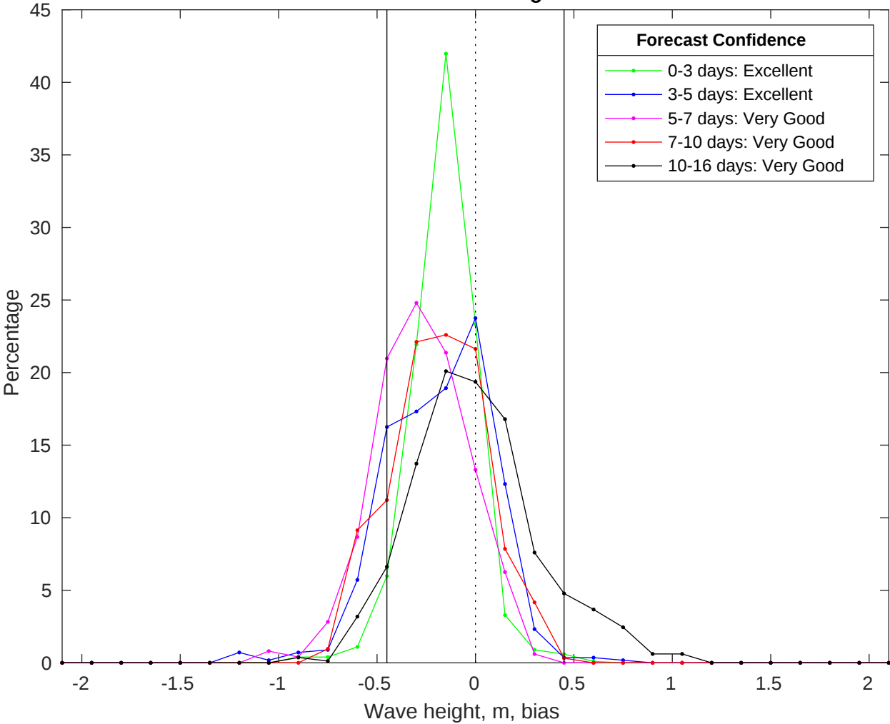
NDBC 42019 vs GFS Waves Bias Histogram: 15-Jul-2025
