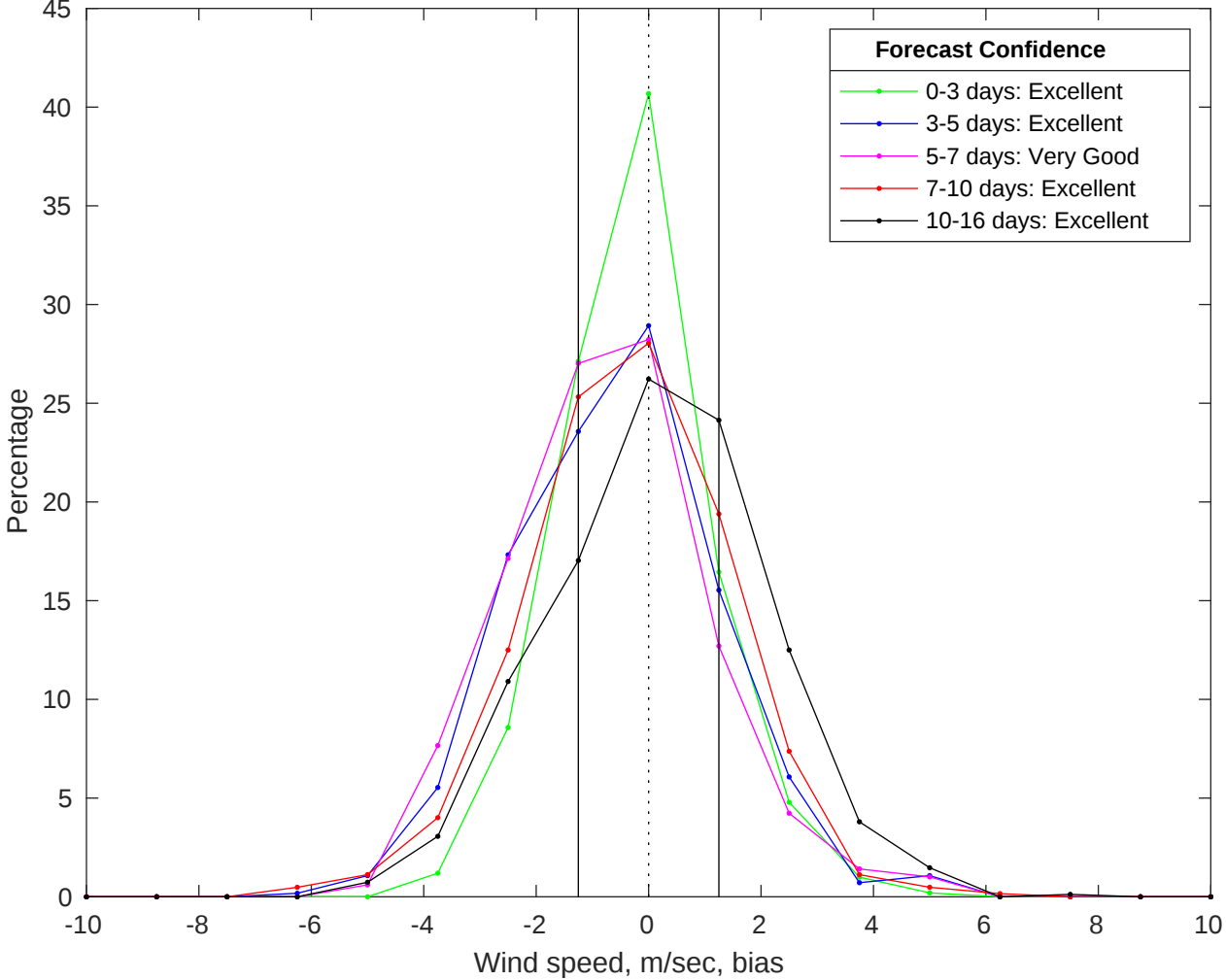
NDBC 42019 vs GFS Winds Bias Histogram: 15-Jul-2025
