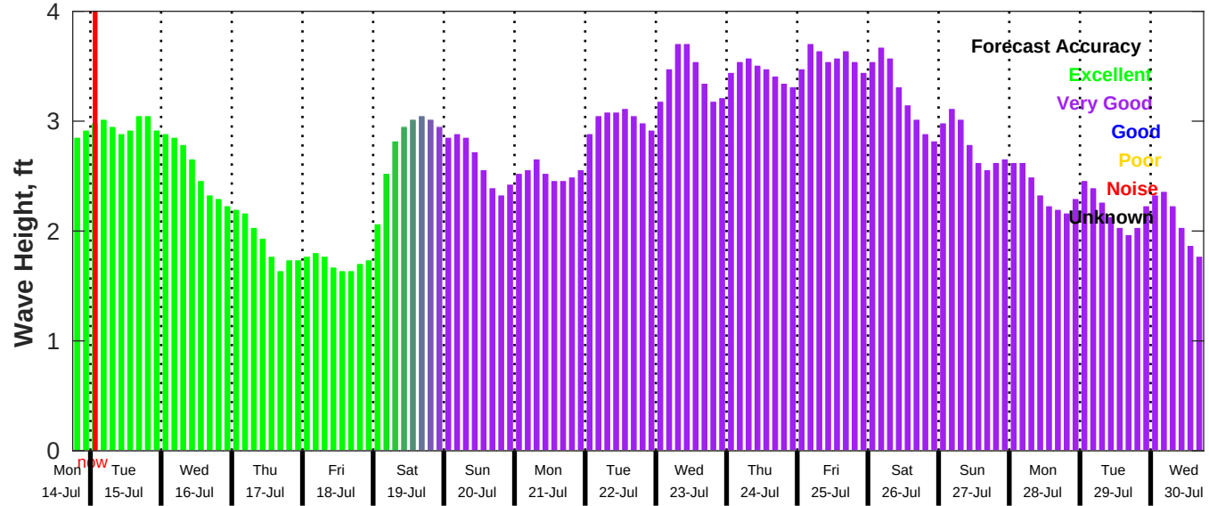
GFS Wave Forecast for NDBC 42019 from 14-Jul-2025 18:00:00 to 30-Jul-2025 18:00:00
