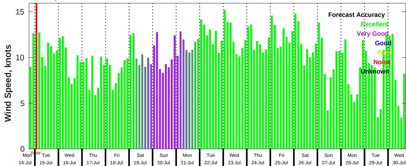
GFS Wind Speed Forecast for NDBC 42019 from 14-Jul-2025 18:00:00 to 30-Jul-2025 18:00:00
