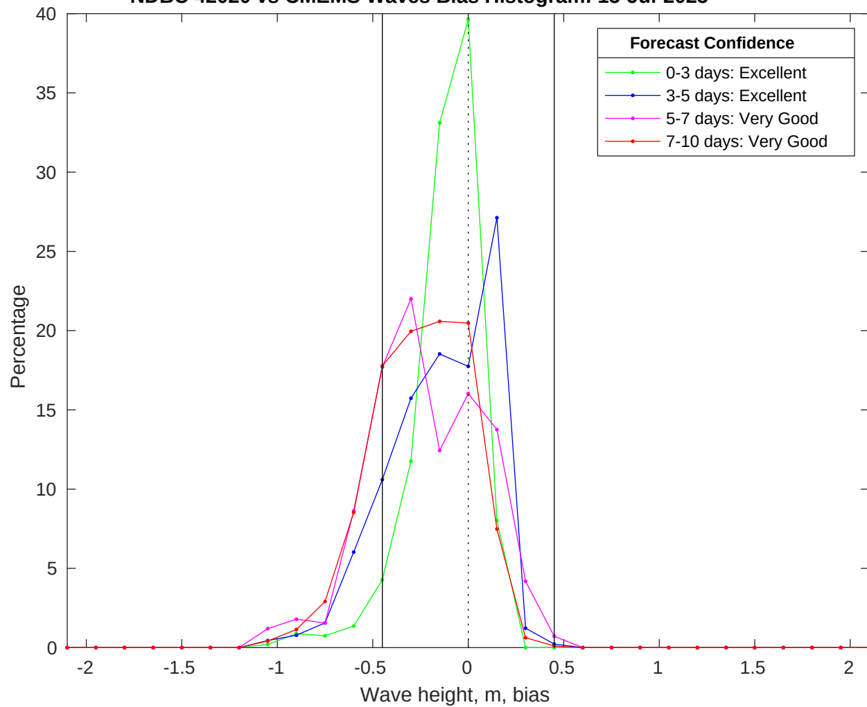
NDBC 42020 vs CMEMS Waves Bias Histogram: 15-Jul-2025
