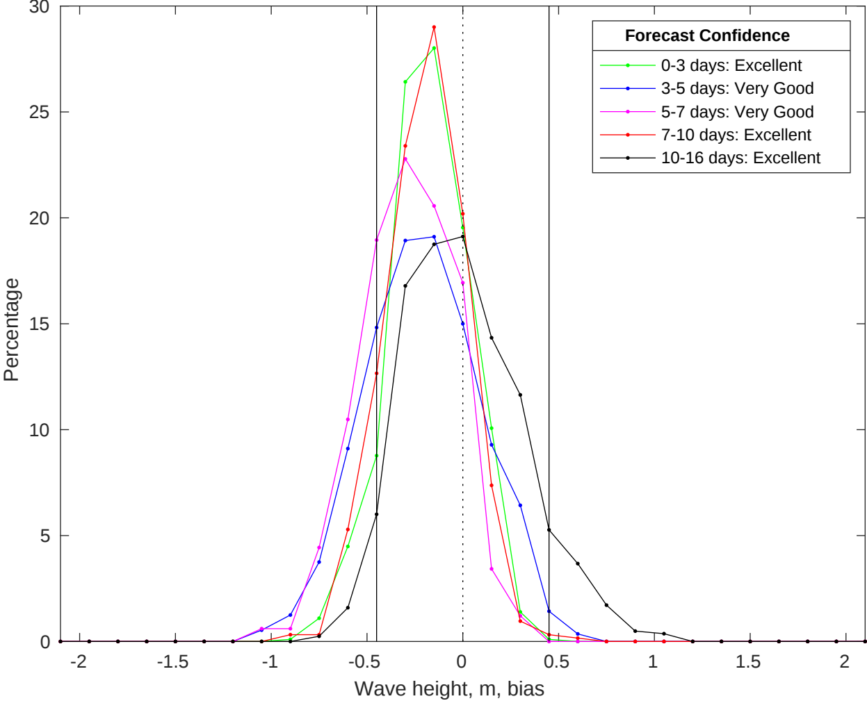
NDBC 42020 vs GFS Waves Bias Histogram: 15-Jul-2025
