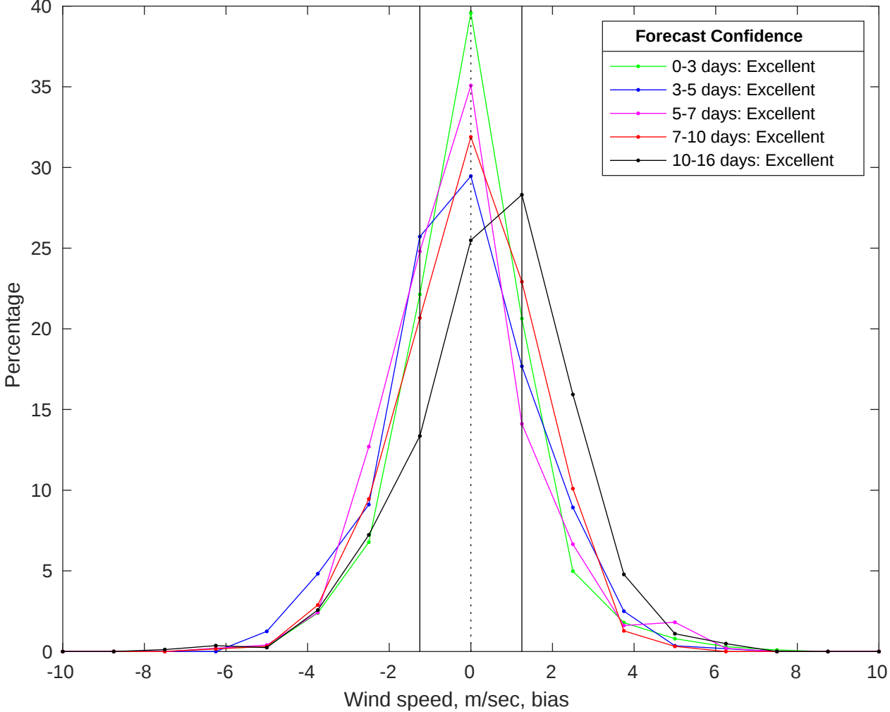
NDBC 42020 vs GFS Winds Bias Histogram: 15-Jul-2025
