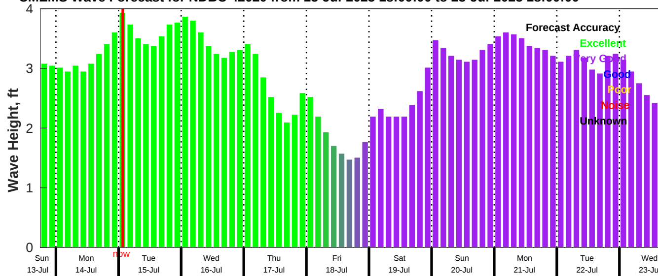
CMEMS Wave Forecast for NDBC 42020 from 13-Jul-2025 18:00:00 to 23-Jul-2025 18:00:00
