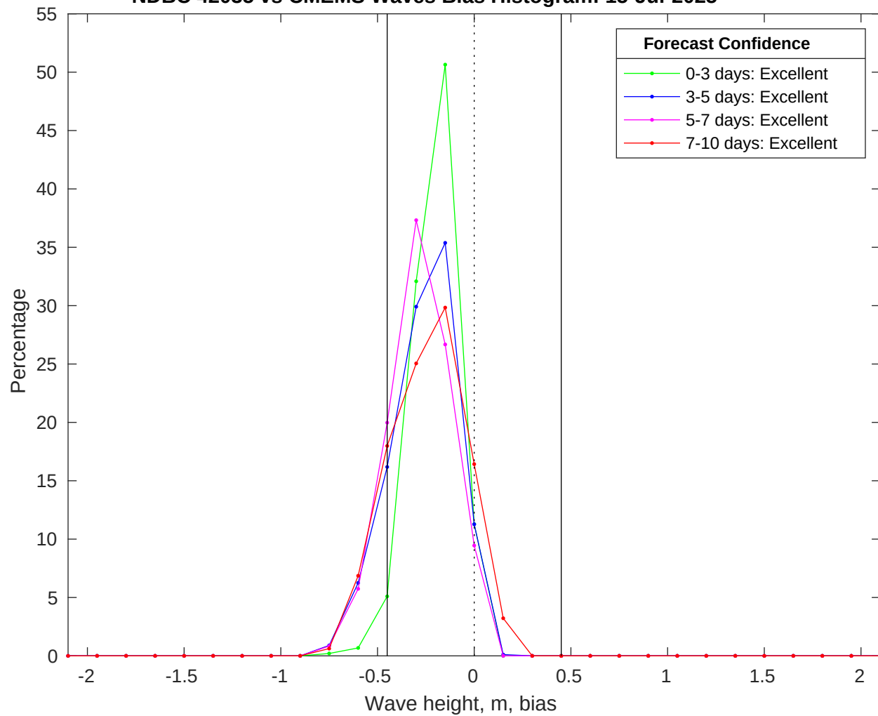
NDBC 42035 vs CMEMS Waves Bias Histogram: 15-Jul-2025
