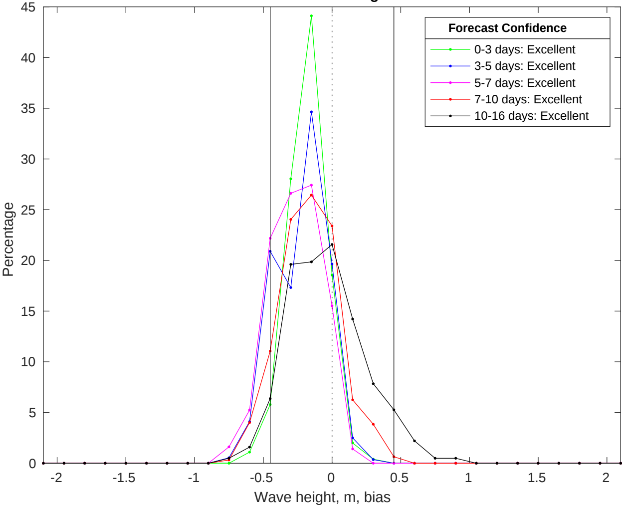
NDBC 42035 vs GFS Waves Bias Histogram: 15-Jul-2025
