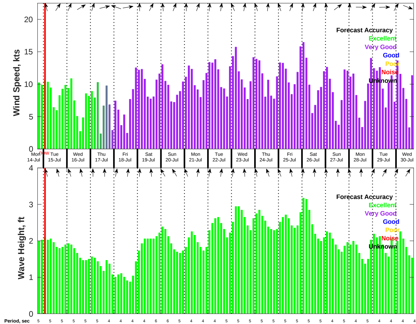
Wind & Wave Forecast for NDBC 42035 from 14-Jul-2025 18:00:00 to 30-Jul-2025 18:00:00
