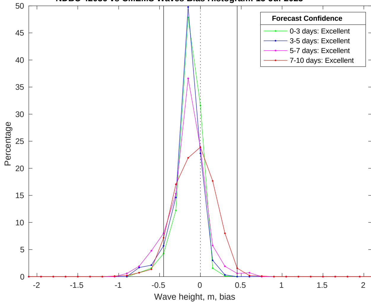
NDBC 42036 vs CMEMS Waves Bias Histogram: 15-Jul-2025
