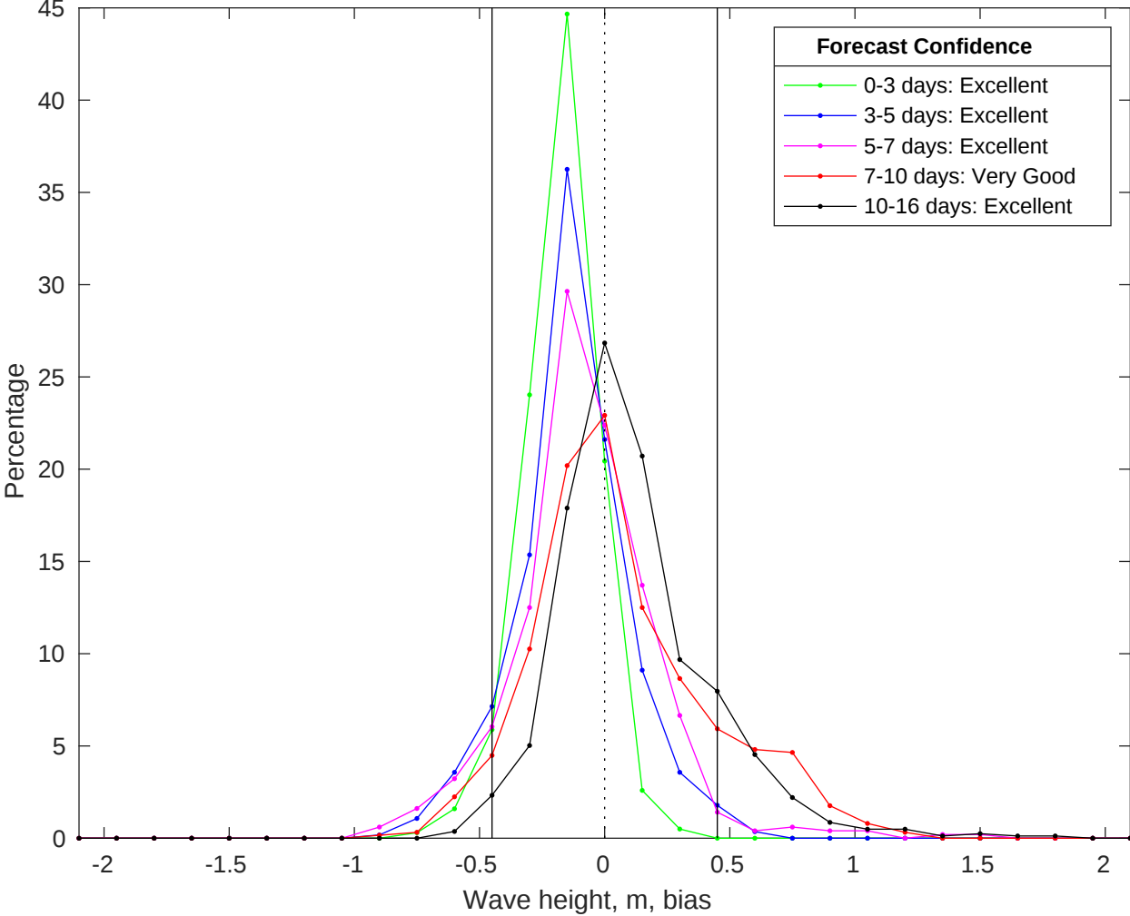
NDBC 42036 vs GFS Waves Bias Histogram: 15-Jul-2025
