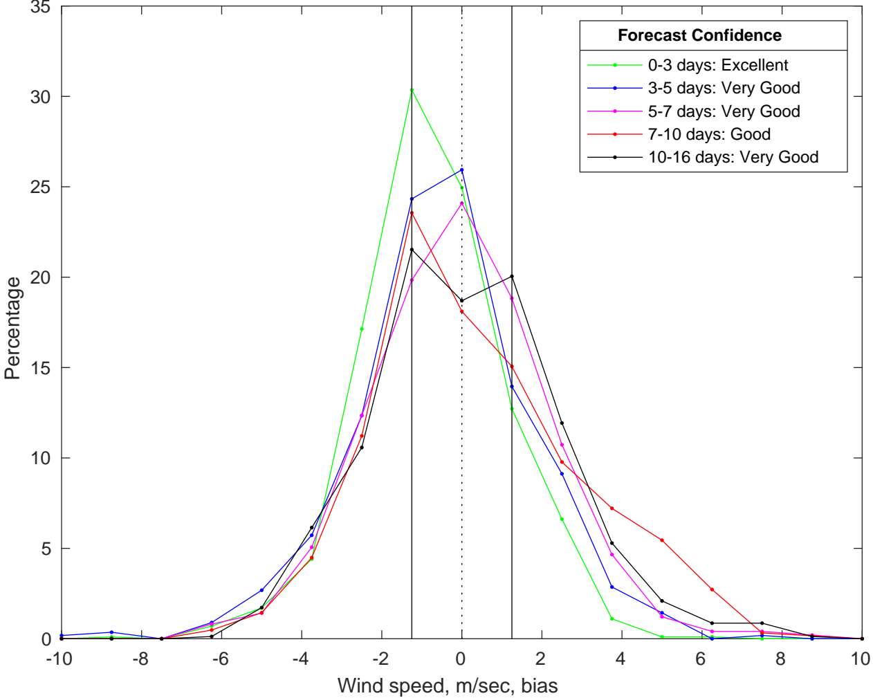
NDBC 42036 vs GFS Winds Bias Histogram: 15-Jul-2025
