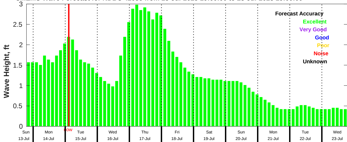
CMEMS Wave Forecast for NDBC 42036 from 13-Jul-2025 19:00:00 to 23-Jul-2025 19:00:00
