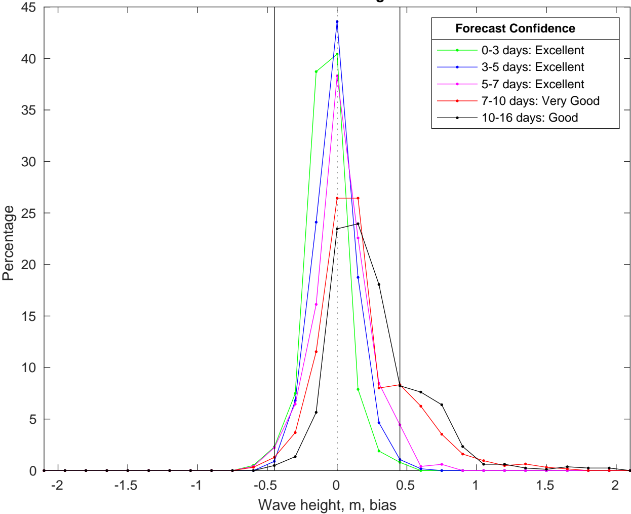
NDBC 42040 vs GFS Waves Bias Histogram: 15-Jul-2025
