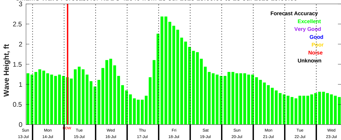
CMEMS Wave Forecast for NDBC 42040 from 13-Jul-2025 19:00:00 to 23-Jul-2025 19:00:00
