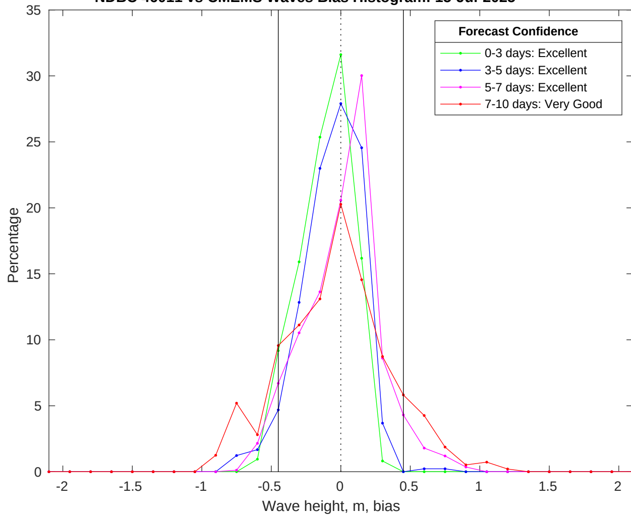
NDBC 46011 vs CMEMS Waves Bias Histogram: 15-Jul-2025
