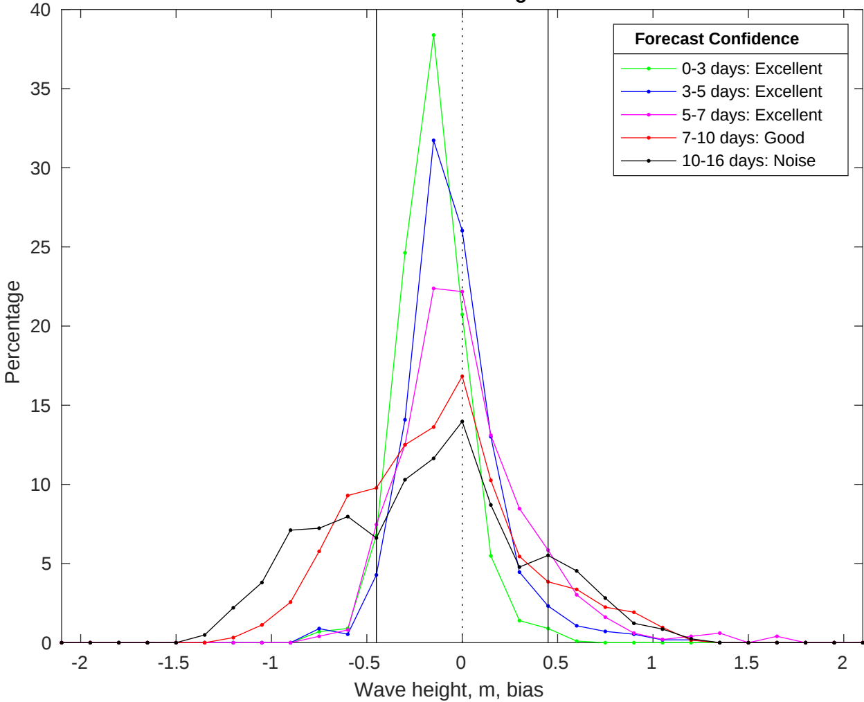
NDBC 46011 vs GFS Waves Bias Histogram: 15-Jul-2025
