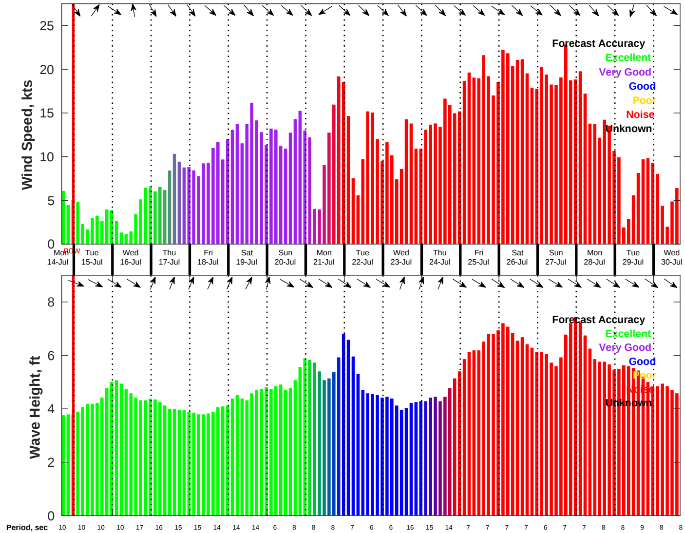
Wind & Wave Forecast for NDBC 46011 from 14-Jul-2025 16:00:00 to 30-Jul-2025 16:00:00
