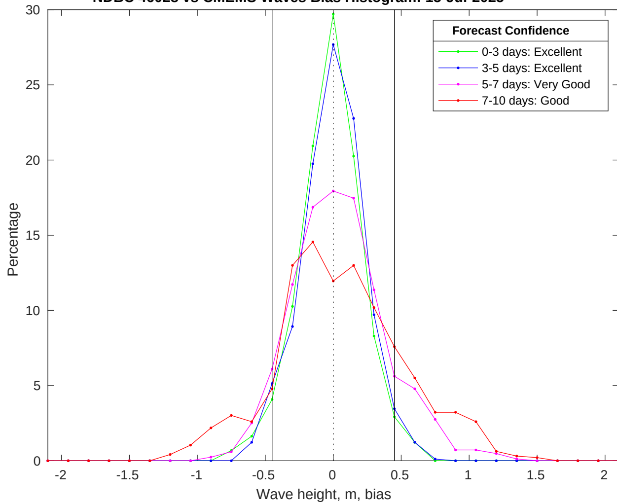
NDBC 46028 vs CMEMS Waves Bias Histogram: 15-Jul-2025
