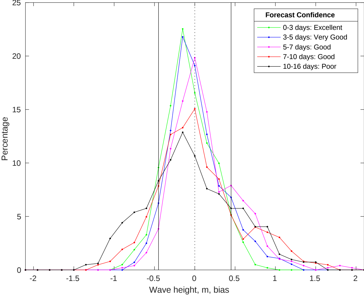
NDBC 46028 vs GFS Waves Bias Histogram: 15-Jul-2025
