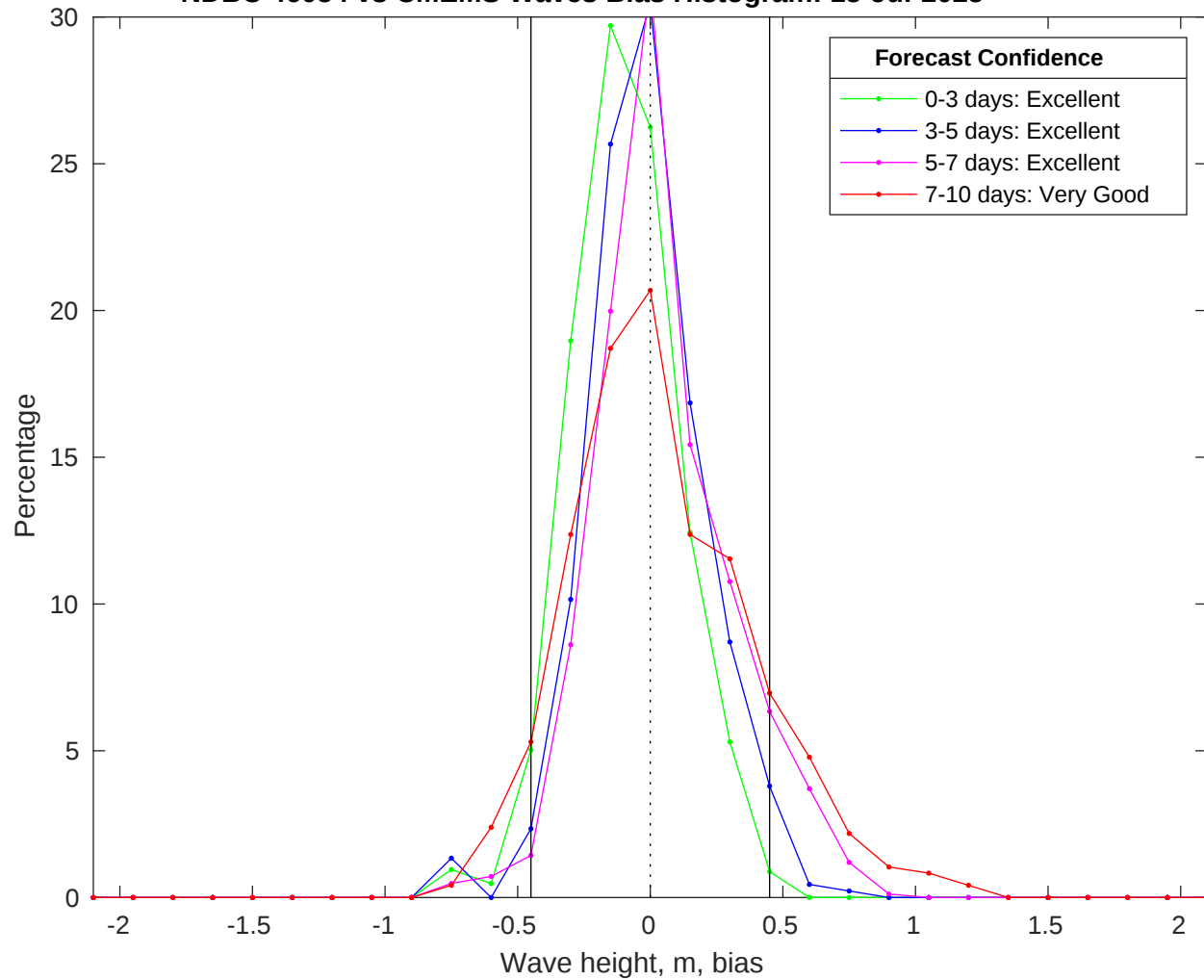
NDBC 46054 vs CMEMS Waves Bias Histogram: 15-Jul-2025
