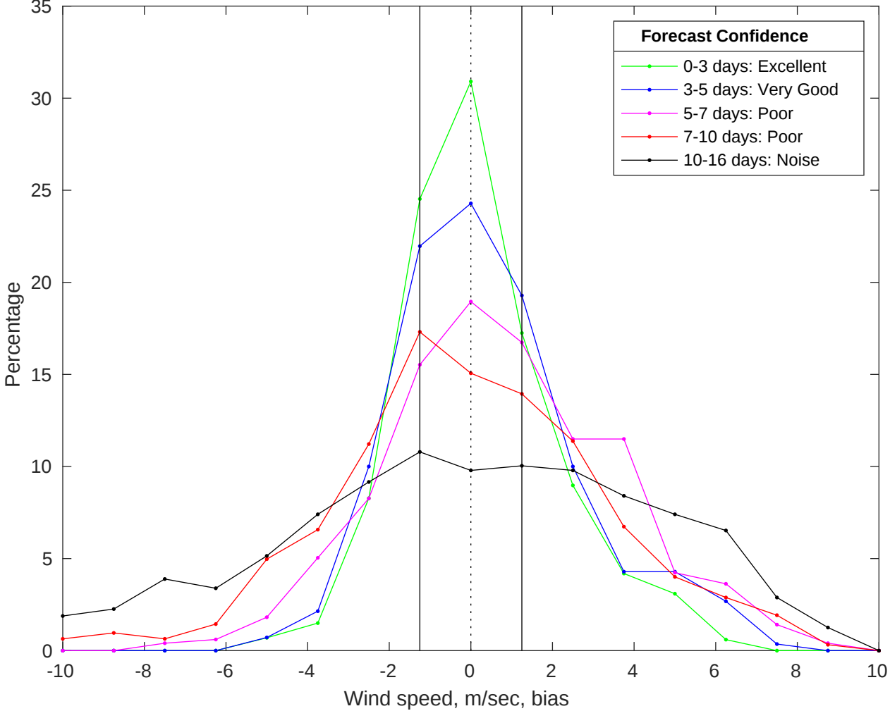
NDBC 46054 vs GFS Winds Bias Histogram: 15-Jul-2025
