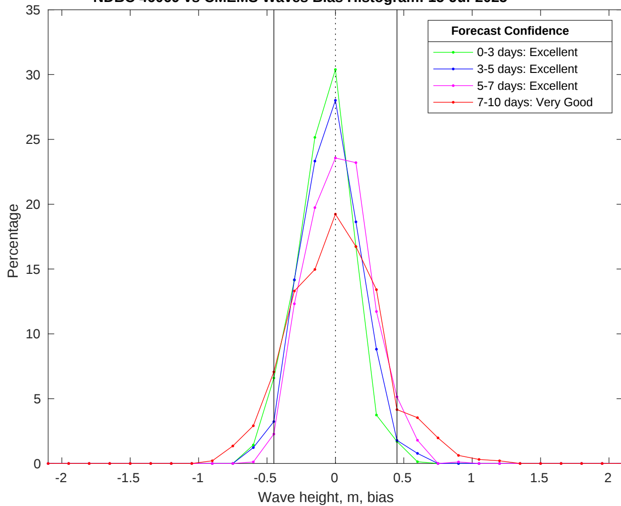
NDBC 46069 vs CMEMS Waves Bias Histogram: 15-Jul-2025
