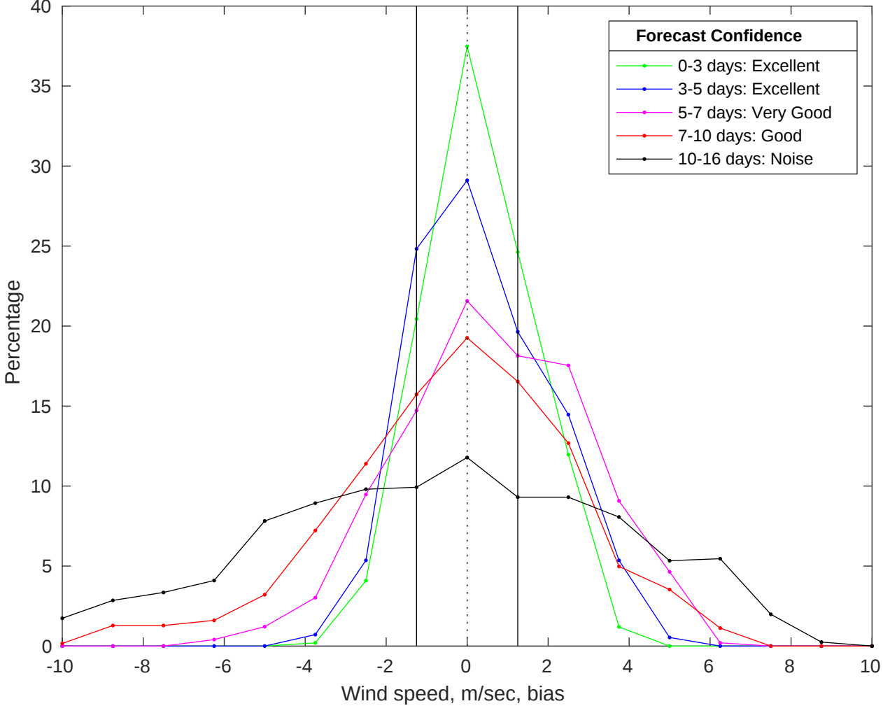
NDBC 46069 vs GFS Winds Bias Histogram: 15-Jul-2025
