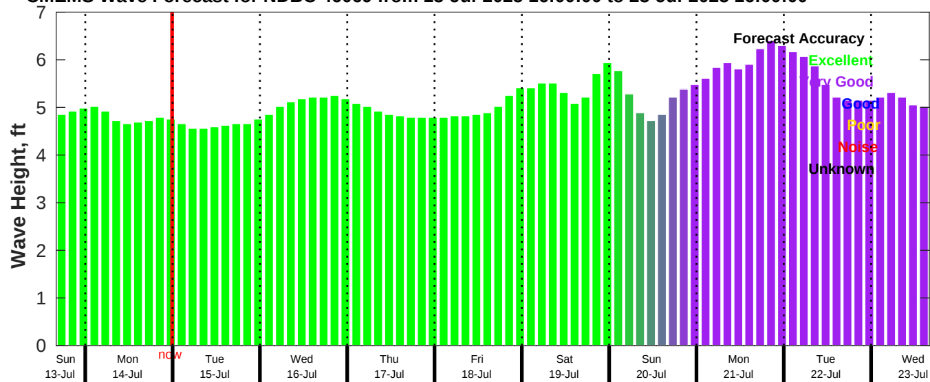
CMEMS Wave Forecast for NDBC 46069 from 13-Jul-2025 16:00:00 to 23-Jul-2025 16:00:00
