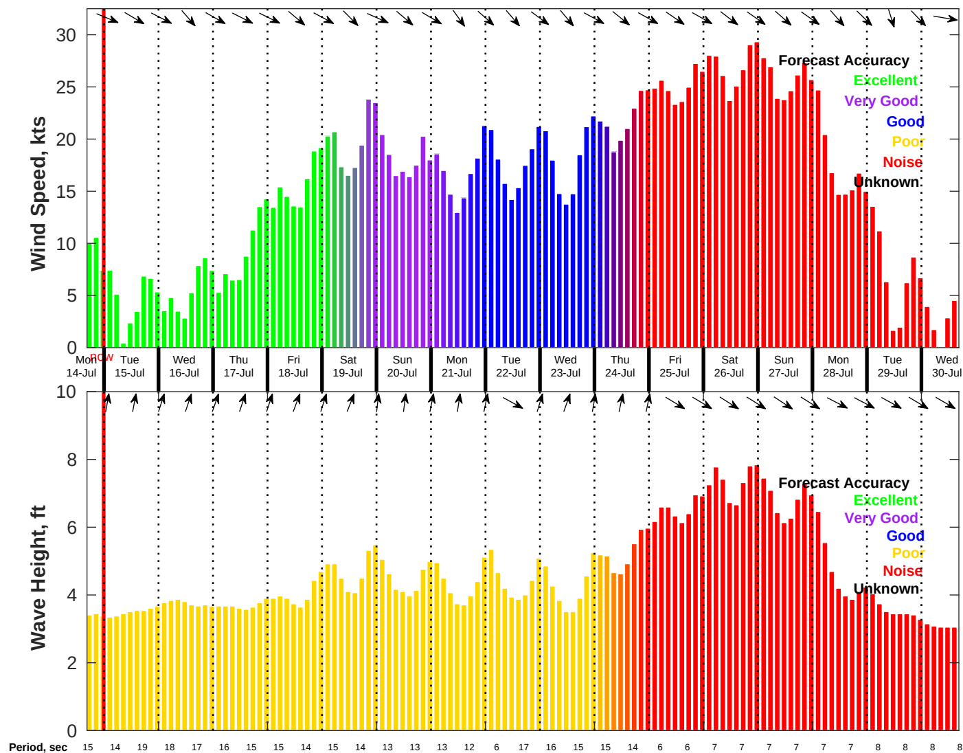
Wind & Wave Forecast for NDBC 46069 from 14-Jul-2025 16:00:00 to 30-Jul-2025 16:00:00
