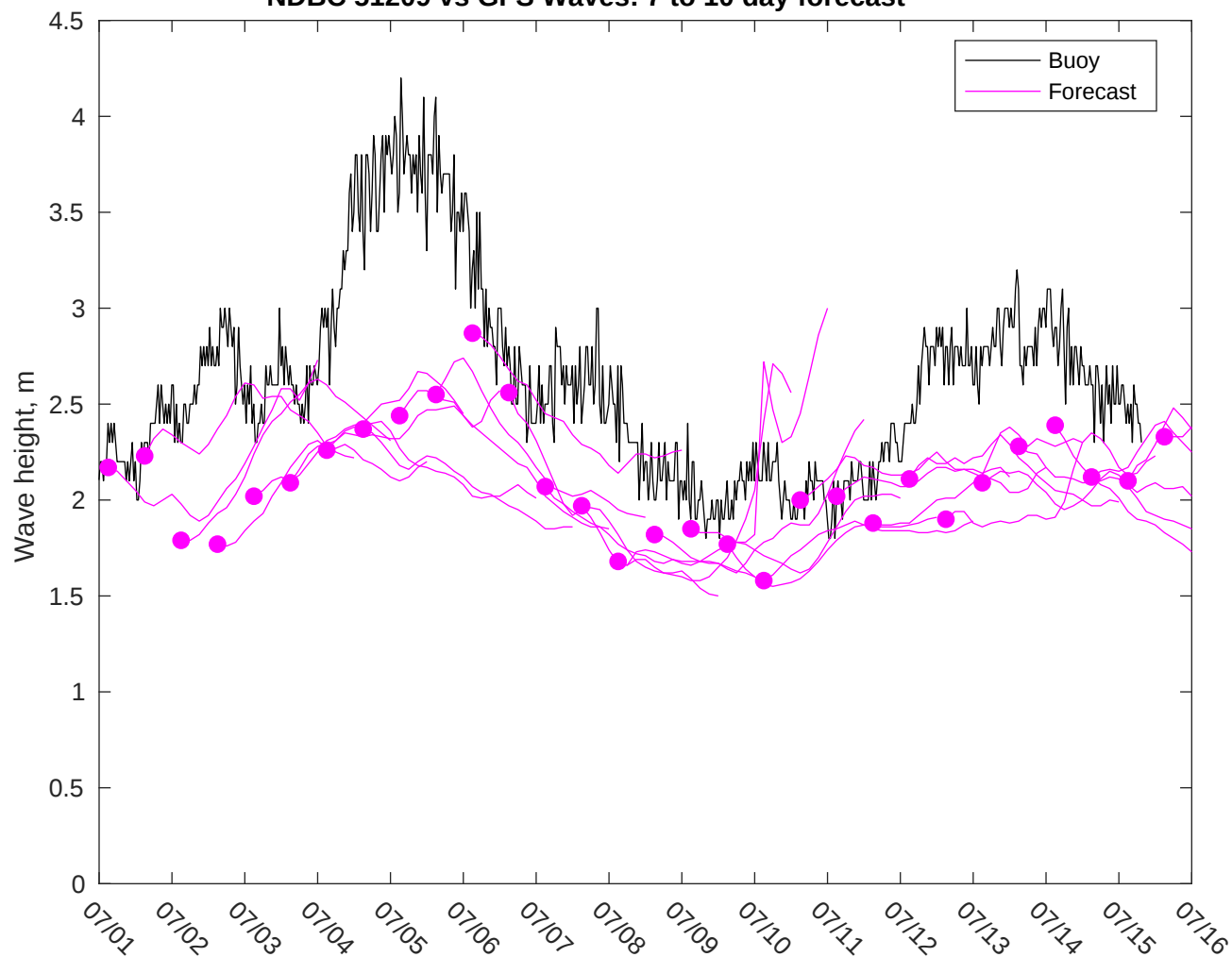
NDBC 51209 vs GFS Waves: 7 to 10 day forecast
