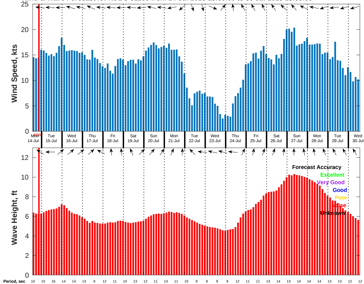
Wind & Wave Forecast for NDBC 51209 from 14-Jul-2025 13:00:00 to 30-Jul-2025 13:00:00
