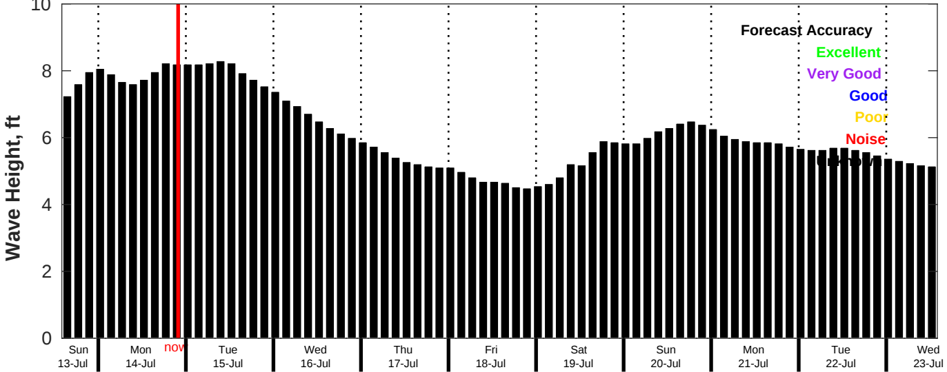
CMEMS Wave Forecast for NDBC 51211 from 13-Jul-2025 14:00:00 to 23-Jul-2025 14:00:00
