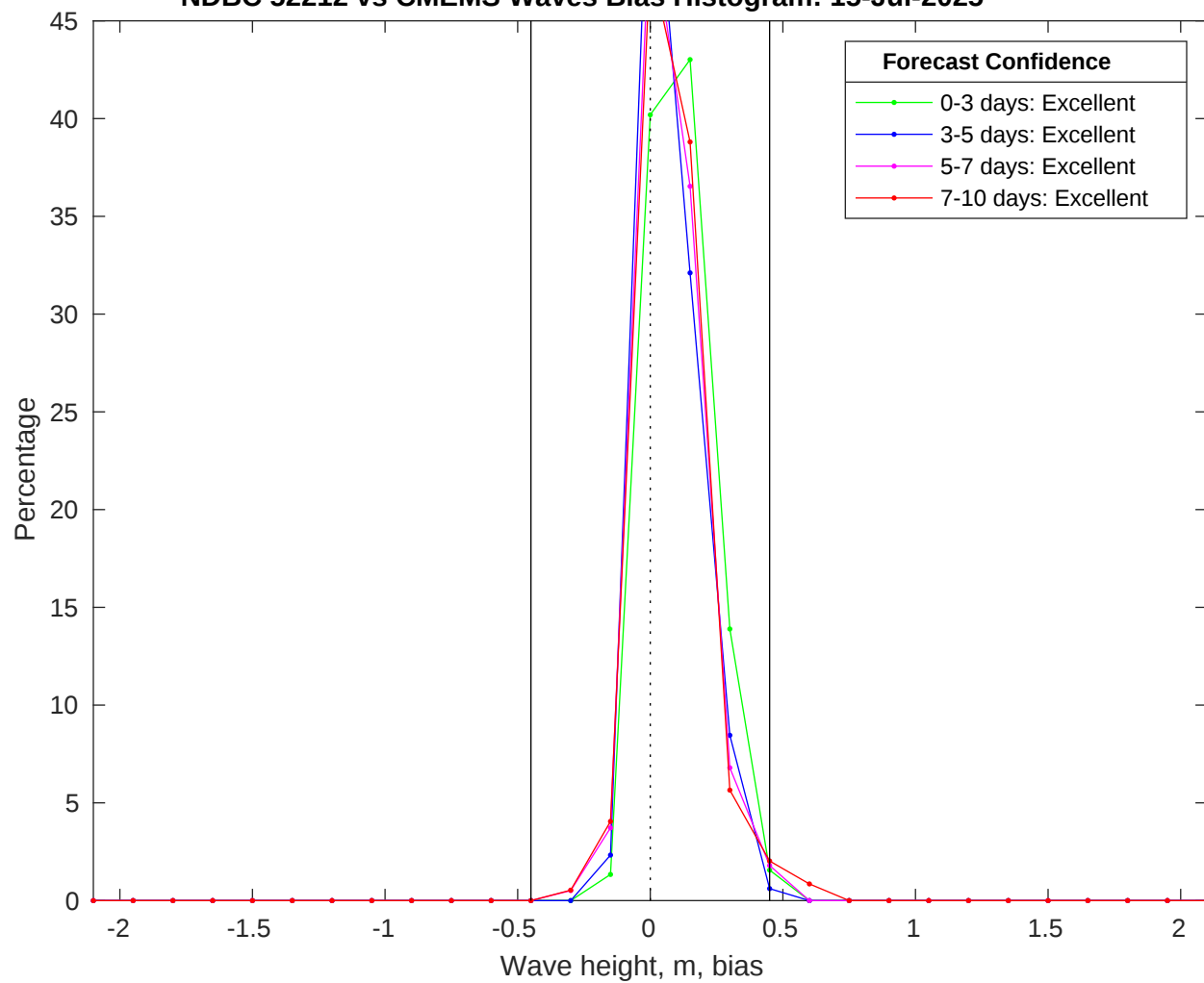
NDBC 52212 vs CMEMS Waves Bias Histogram: 15-Jul-2025
