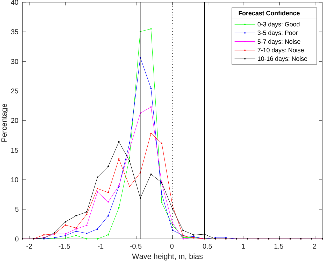
NDBC 52213 vs GFS Waves Bias Histogram: 15-Jul-2025
