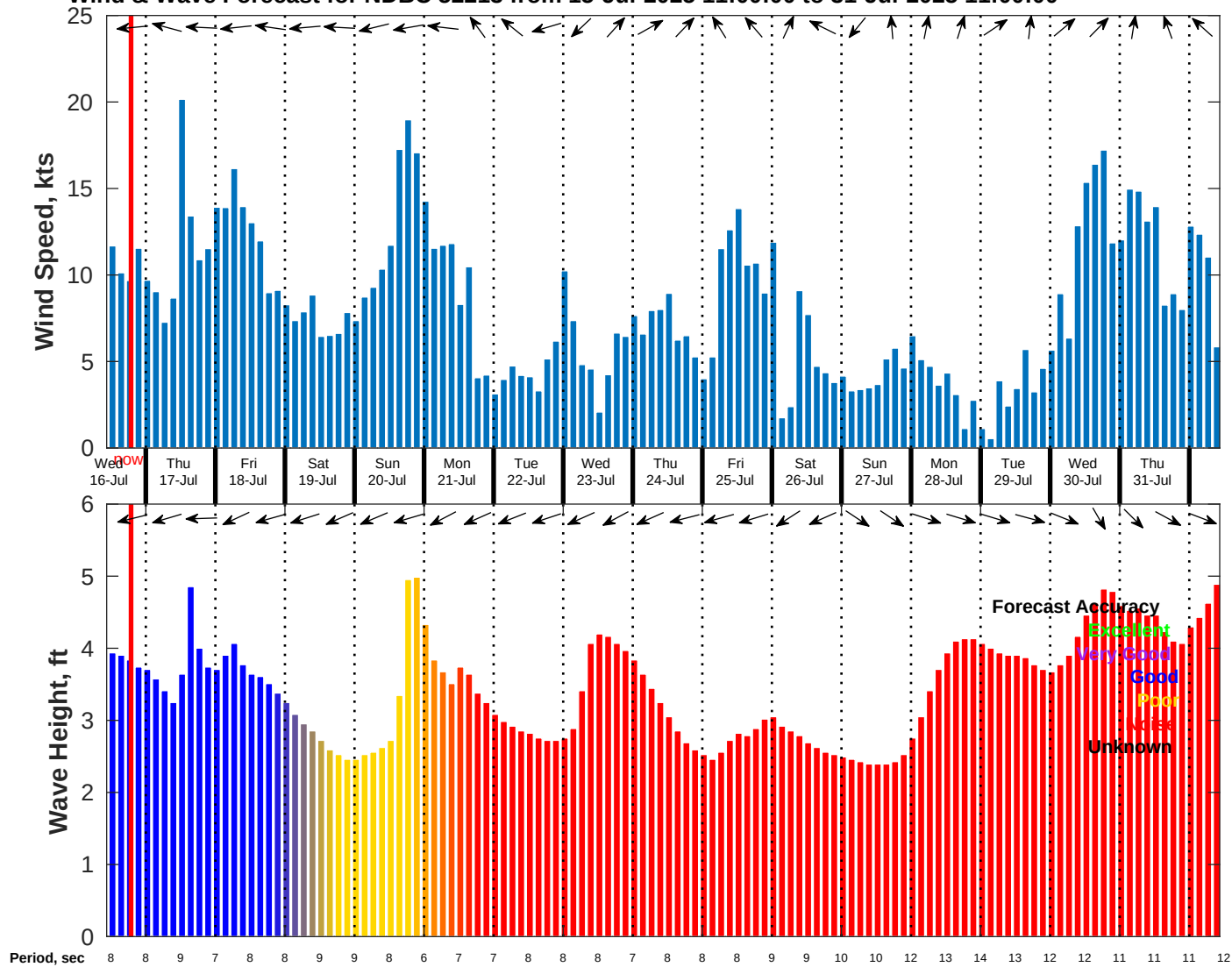
Wind & Wave Forecast for NDBC 52213 from 15-Jul-2025 11:00:00 to 31-Jul-2025 11:00:00
