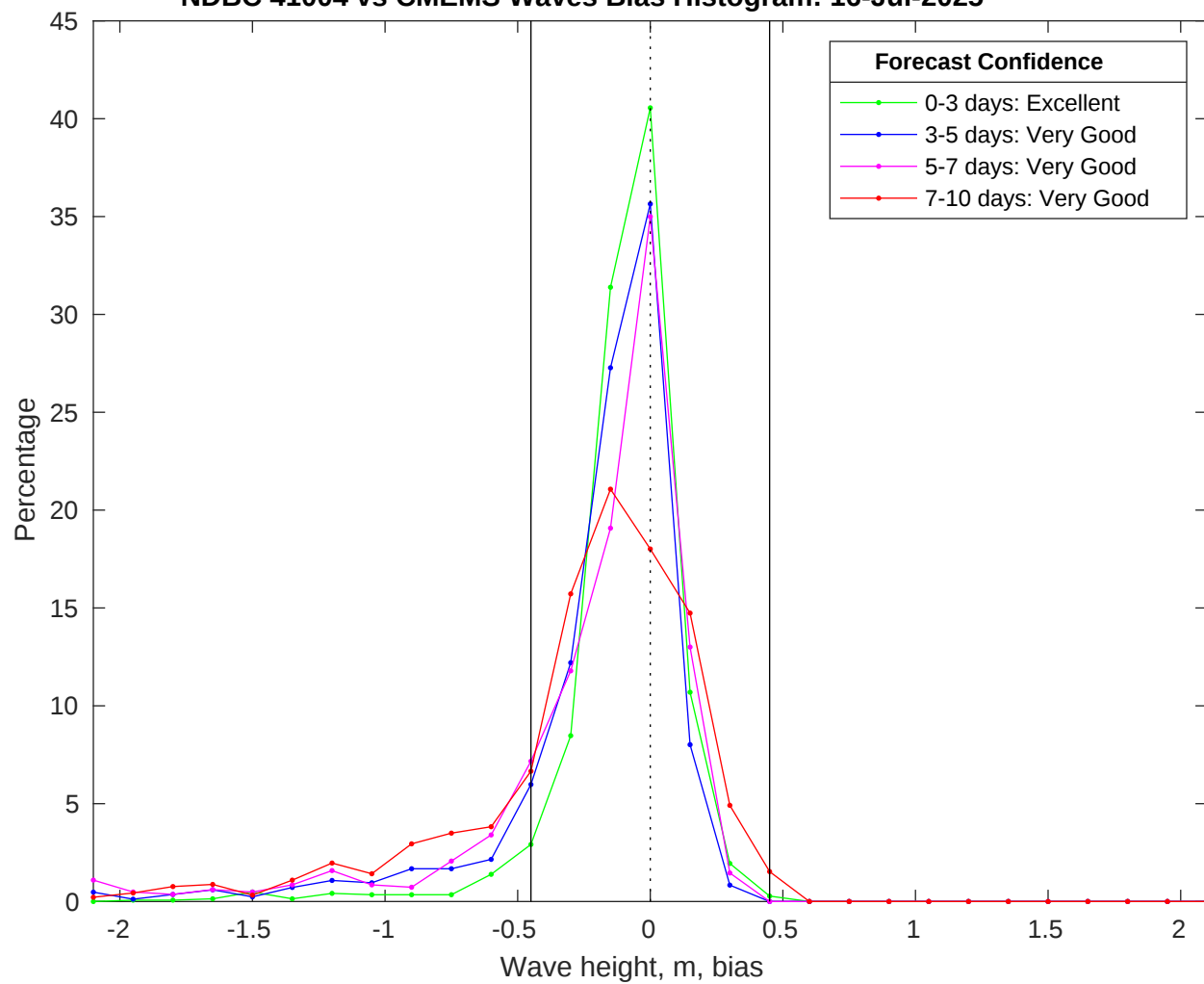
NDBC 41004 vs CMEMS Waves Bias Histogram: 16-Jul-2025
