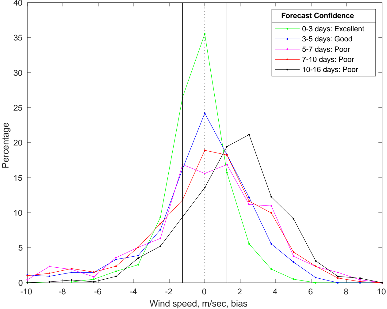
NDBC 41004 vs GFS Winds Bias Histogram: 16-Jul-2025
