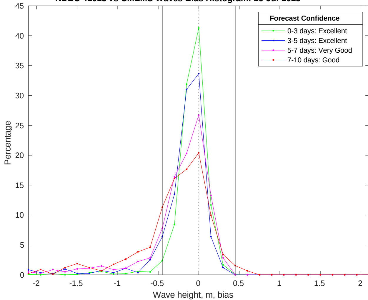
NDBC 41013 vs CMEMS Waves Bias Histogram: 16-Jul-2025
